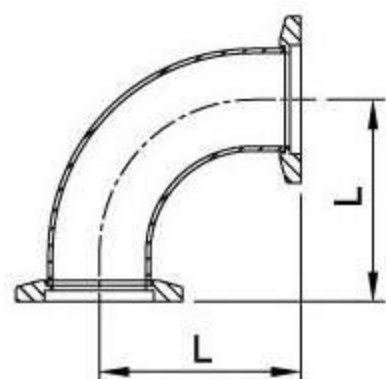
90° Elbow Flange
