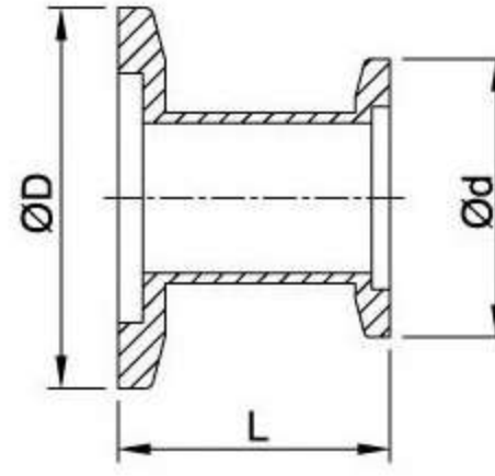
Straight Reducer
