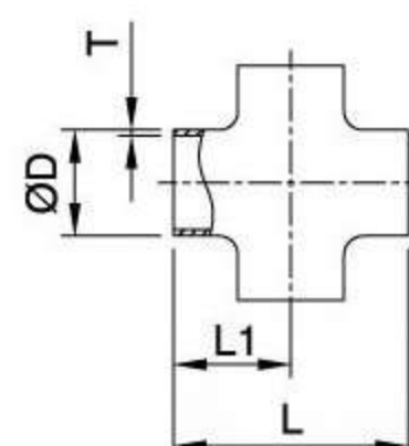
Cross
