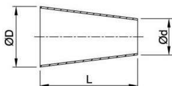
Concentric Reducer
