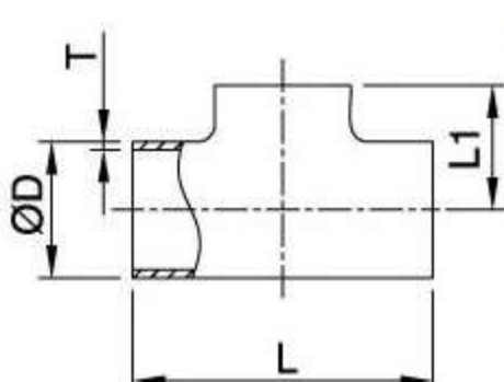
Welding Tee
