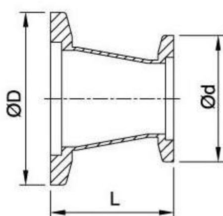
Conical Reducer
