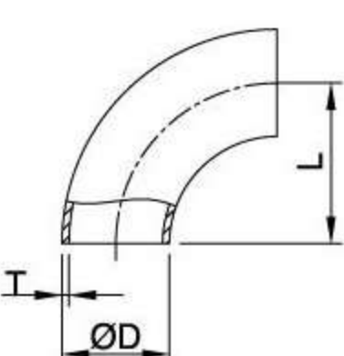
90° Short Elbow
