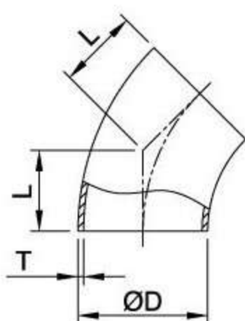
45° Short Elbow
