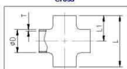
Cross
