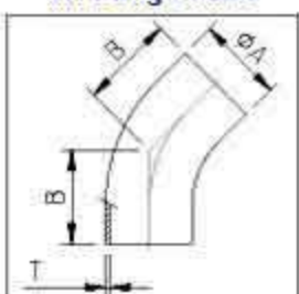
C.L2KS-45° Elbow
