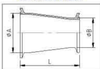
C.31-14MP Concentric Reducer Clamp End
