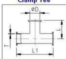
Clamp Tee
