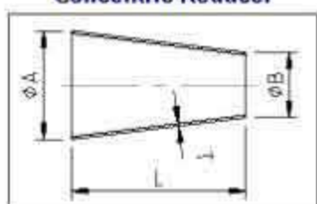
C.L31-Concentric Reducer
