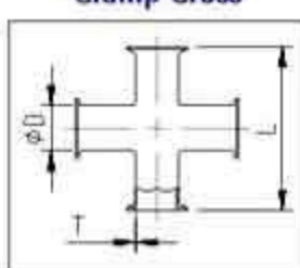
Clamp Cross
