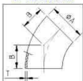
C.2WK-45° Elbow
