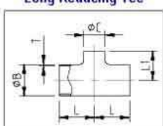
Long Reducing Tee
