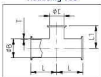
Reducing Tee
