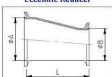
C.32-14MP Eccentric Reducer Clamp End
