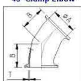
C.2KMP-45° Elbow
