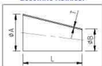
C.L32-Eccentric Reducer
