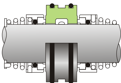
22mm Centre Collets in Carbon Face /SS face/TC Face
