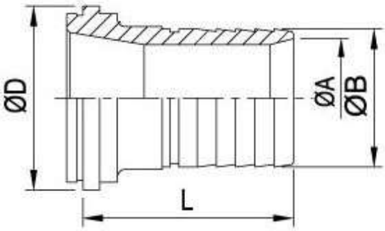
Mancon Liner 14 Hose Adapter
