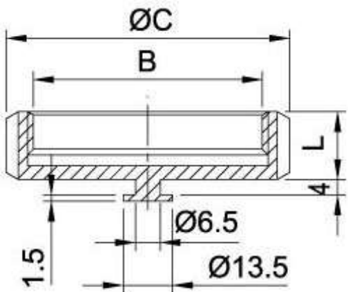
Mancon Blank Nut 4 Slots M-13RBN
