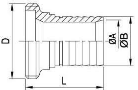
Mancon Male 15AHR Hose Adapter
