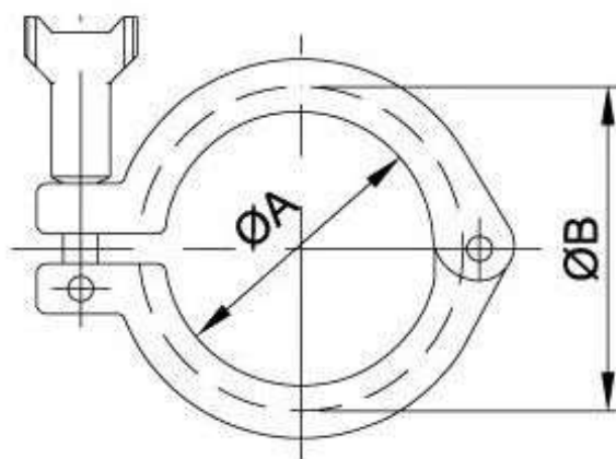
13IS I-line Clamp
