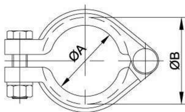
13IU Bolted Clamp
