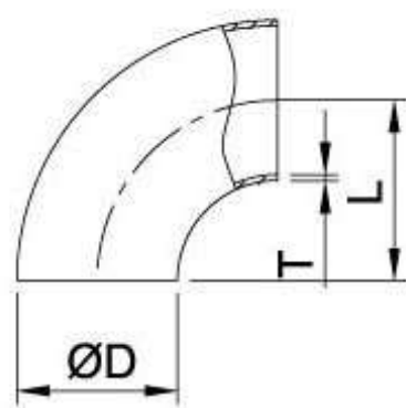
90° Short Tube Bend
