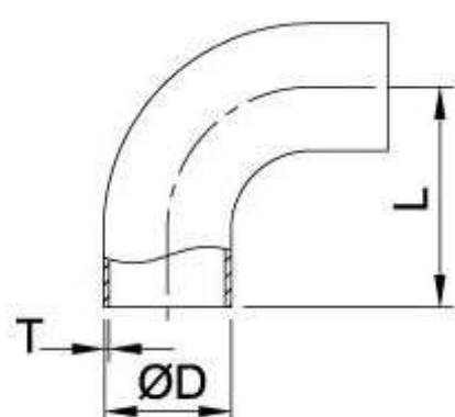
90° Long Tube Bend
