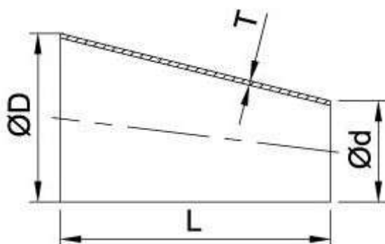
Eccentric Reducer
