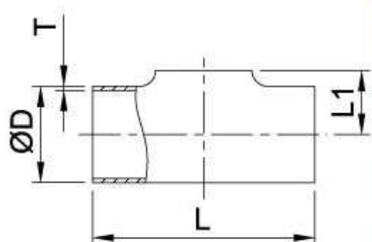
Pull Tee
