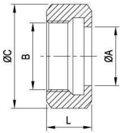
3A Hexagonal Nut 3A-13H
