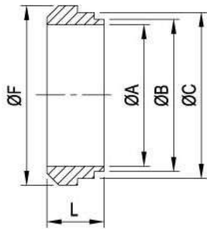
3A short Bevel Seat Weld Liner 3A-14PRF
