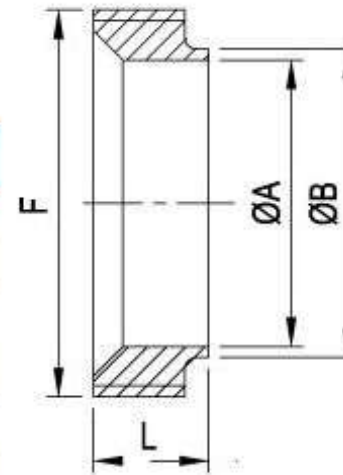
3A short Bevel Seat Weld Male 3A-15TRF
